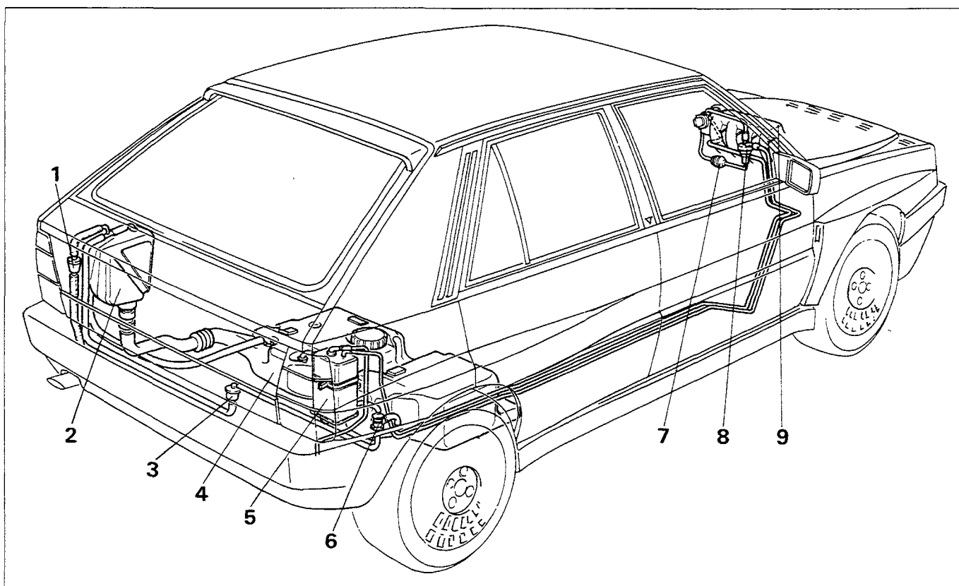
Diagram showing fuel evaporation control system on vehicle
